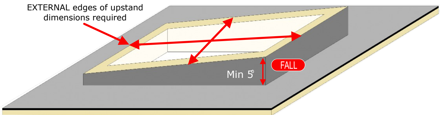
UPSTAND DETAIL
