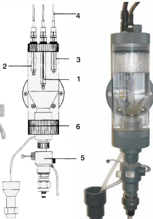
5 AAA7000 Flow Switch
