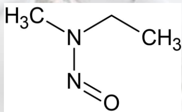
N-Nitrosomethylethylamine
