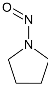
1-Nitrosopyrrolidine
