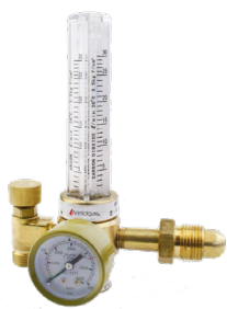
0-25 L/MIN Flowmeter Argon/Co2 Regulator Part No: GAS0017
