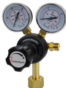
Single stage 2G Co2 Regulator 10 Bar (Female Fitting) Part No: GAS0004
