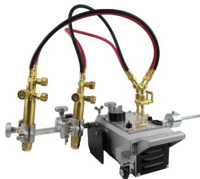
Twin Torch Kit (Machine not included) Part No: GAS0067
