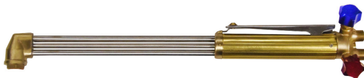
18/90 ECO Cutting Torch - NM250 Part No: GAS2005
